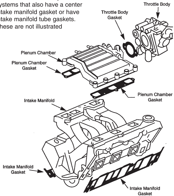
Typical V6 / V8 E.F.I. System
